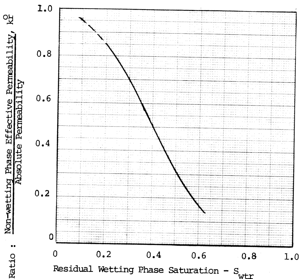
Figure 9. Average curve showing effect of residual wetting phase saturation on effective permeability of non-wetting phase.
