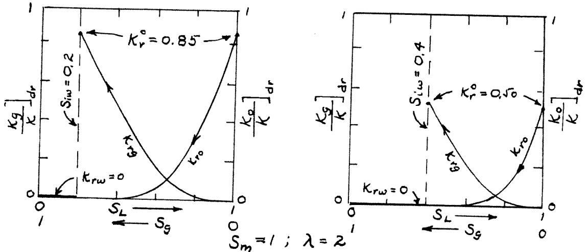
Figure 13 Three-phase drainage relative permeability curves
