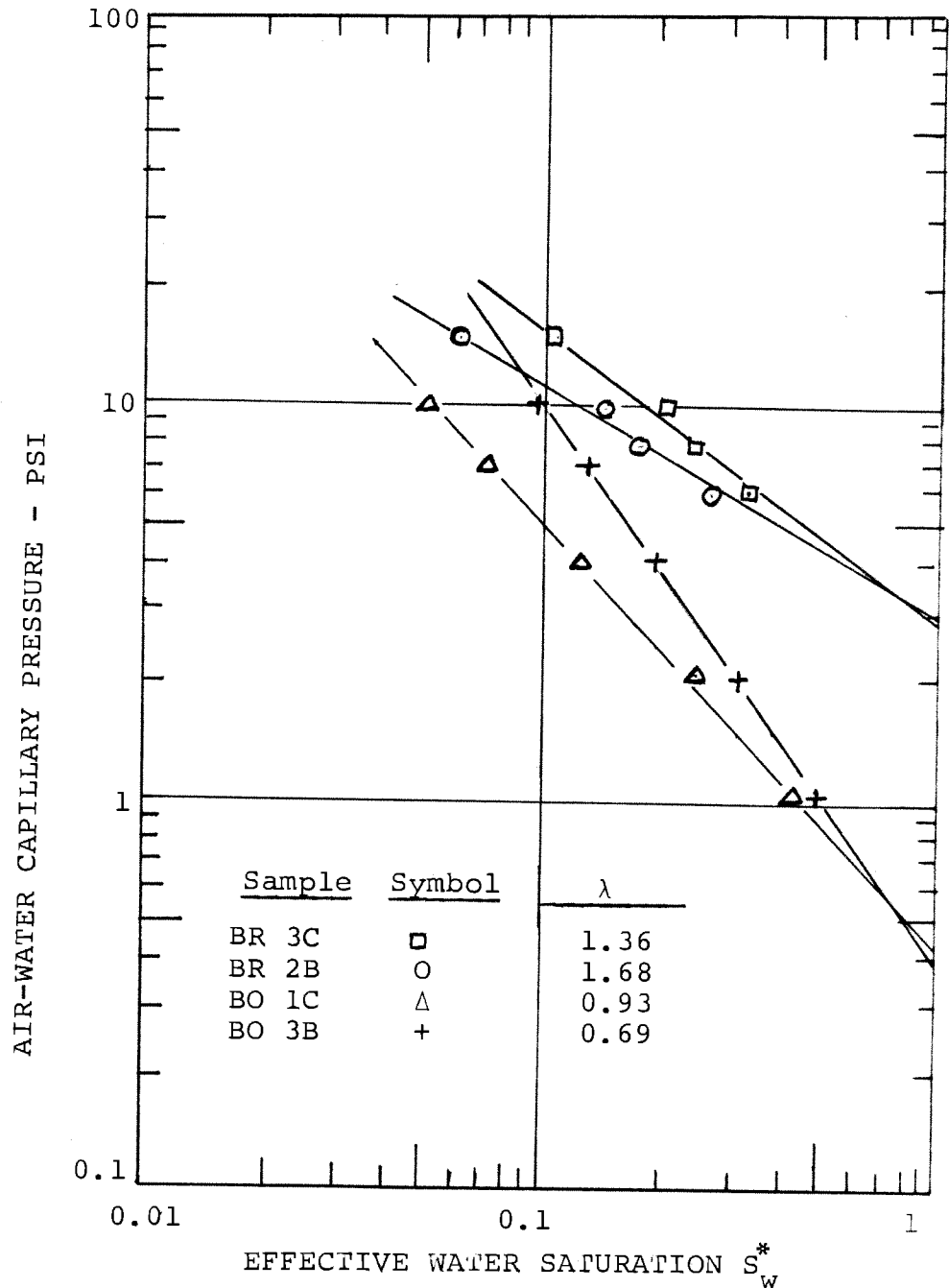
Figure 6. Log-Log Relationship of Capillary Pressure and Effective Water Saturation.
